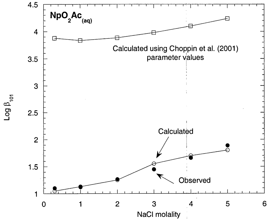
Figure 1. \text{Log } \beta_{101} versus NaCl molality for \text{NpO}_2\text{Ac}_{(aq)} . Filled circles: values from Choppin et al. (2001, Tables 20-25); open squares: model predictions calculated using \mu^0/RT(\text{NpO}_2\text{Ac}_{(aq)}) and \lambda(\text{NpO}_2\text{Ac}_{(aq)} - \text{Cl}^-) values listed in Choppin et al. (2001); open circles: model predictions calculated using \mu^0/RT(\text{NpO}_2\text{Ac}_{(aq)}) and \lambda(\text{NpO}_2\text{Ac}_{(aq)} - \text{Cl}^-) values calculated in this work.
